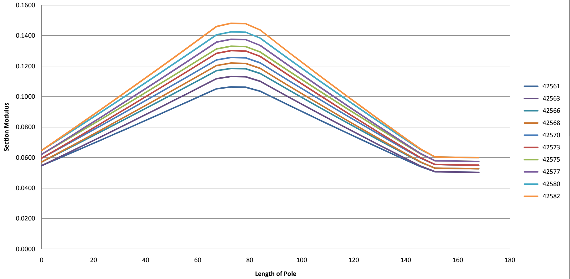
Section Modulus Along Length of Pole
